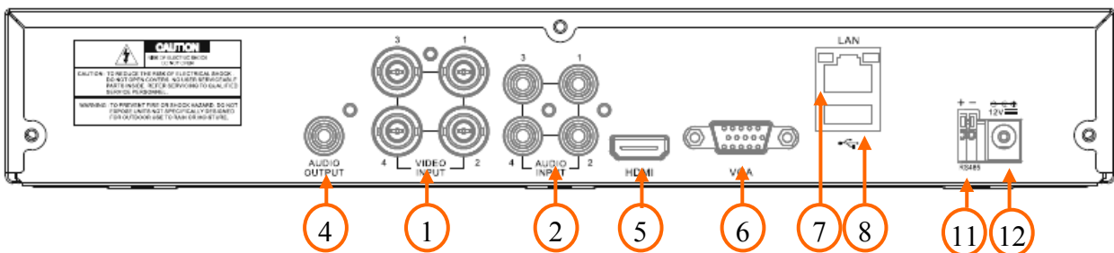
NHDR-3108AHD-II
